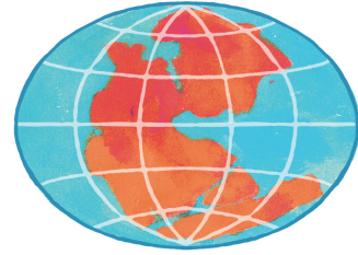
225 million years ago
