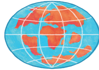
65 million years ago
