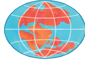
200 million years ago
